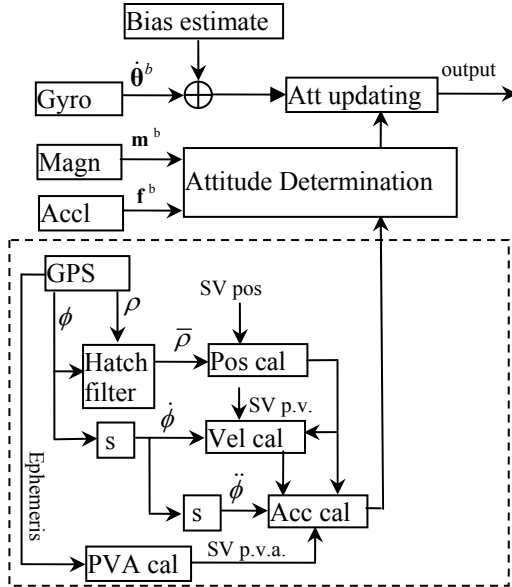
Fig. 2 Structure of the AHRS/GPS system
